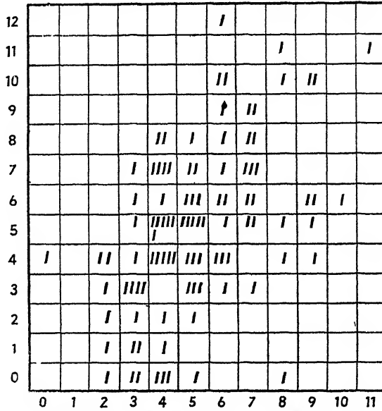
FIG. XIII. Scatter Diagram Correlation of approximately +0.5.
